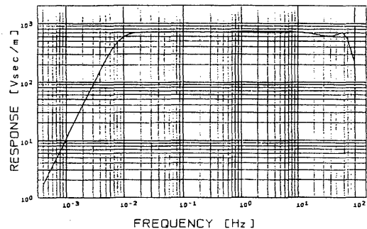
Fig.2 Velocity response curve of STS-2 seismograph
