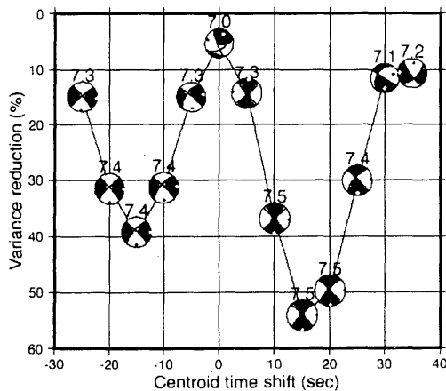
Fig.4 Variance reduction diagram corresponding to each centroid time shift ( \tau ) for the same earthquake as in Fig.3. Each focal mechanism and M_w value is shown on the corresponding to the \tau value. Although the optimal solution is obtained at \tau = 15 sec, the local minimum variance reduction is found at \tau = -15 sec, revealing an inverted mechanism solution.
