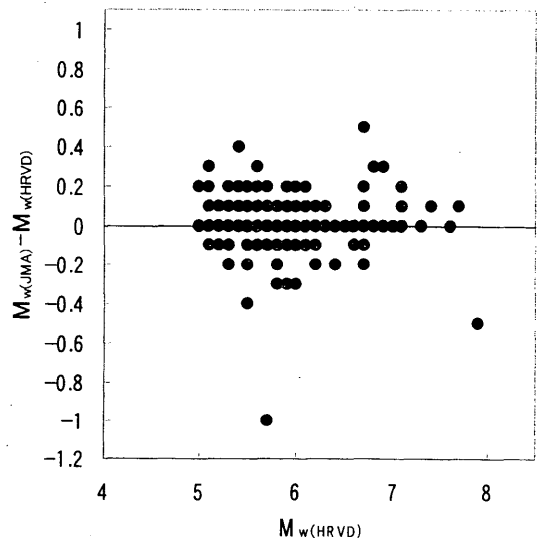
Fig.7 Distribution of moment magnitude difference M_w(JMA)-M_w(HRVD) against M_w(HRVD) , where M_w(JMA) represents the moment magnitude determined by JMA, and M_w(HRVD) is the one determined by Harvard University.
