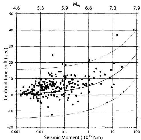
Fig.5 Distribution of the centroid time shift (coordinate) against seismic moment (abscissa). The top horizontal scale shows M_w corresponding to the bottom scale of seismic moment ( 10^{19} \text{Nm} ). The solid curve shows the formula(5) in the text and the dotted curves reveal the 15 second shift below and above the solid curve.
