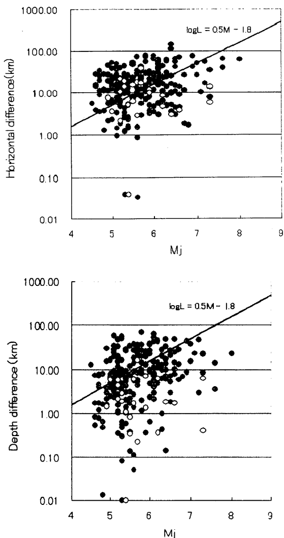
Fig.15 Spatial distances between centroid locations and hypocenters.
