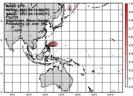
(b) Probability of significant wave height over 6m.
