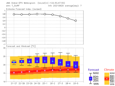
Figure 4.8.5: Meteoagram of the Global EPS for temperature. The upper graph is an EFI timeseries representation, and the lower one is a timeseries representation of forecast ranges with cold color box-and-whisker plots and climatological values with warm shading.
